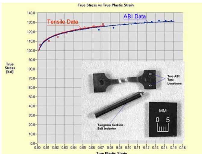
Fig. 2(b) Comparison of true-stress versus true-plastic-strain curves from ABI and tensile tests of high strength steel. (1 ksi = 6.895 MPa). The inset photo shows a tensile specimen and 1.57-mm (0.062-in) diameter tungsten carbide indenter.
