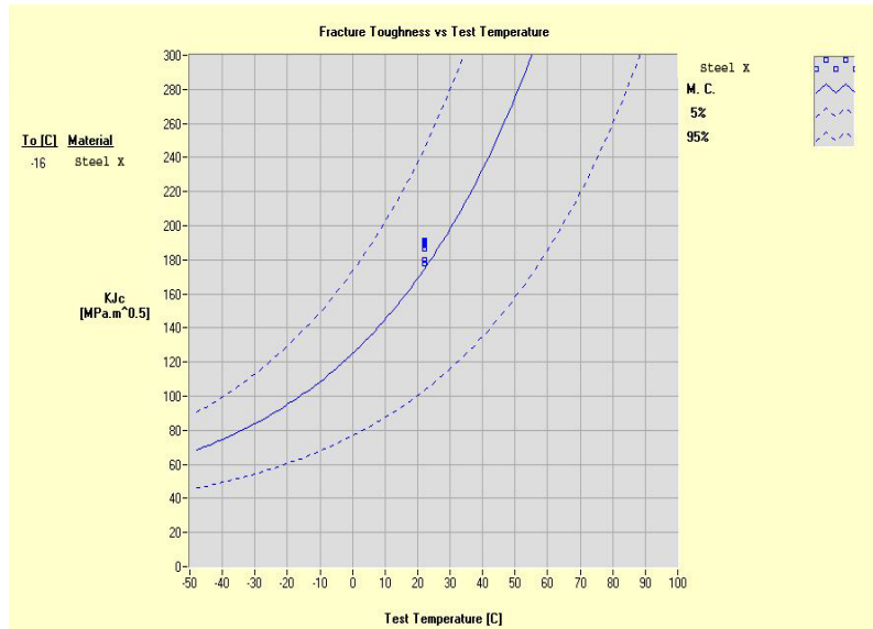
Fig. (5) The ABI-determined fracture toughness values, median curve, and the 95% and 5% confidence limit curves obtained from 15 ABI tests at ambient temperature at 4 pipeline locations. The ABI-determined T_0 value for the Kerosene pipeline is -16^{\circ}\text{C} .
