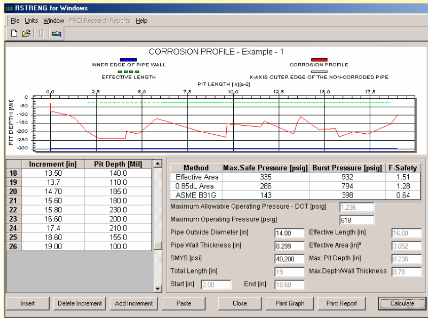
Fig. (7) A few corrosion pits over a 19-inch long section reduced the maximum safe operating pressure from 618 psi (when no corrosion pitting exists) to 143 psi according to the ASME B31G Code.
