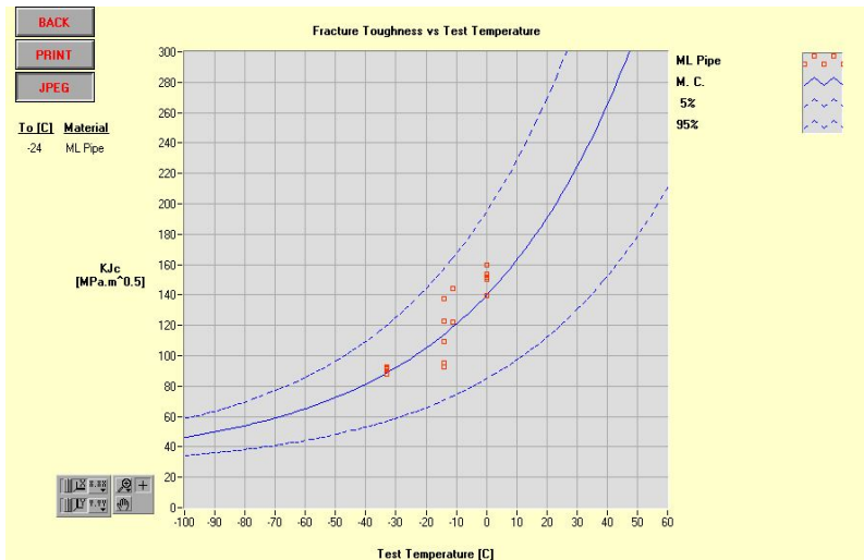
Fig. 4 Static fracture toughness ( K_{Jc} ) values determined from 17 ABI tests conducted on a pipeline steel sample at four test temperatures. The median fracture toughness curve and the 95% and 5% confidence limit curves are shown in the figure.
